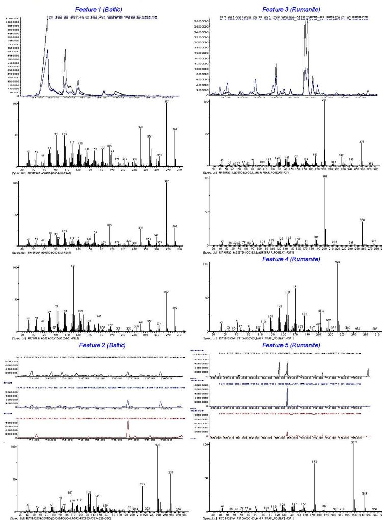
Figure 3. Rumanite and Baltic amber markers: Feature 1 and 2 (Baltic), Feature 3, 4 and 5 (Rumanite)
