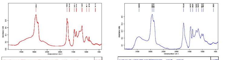
Figure 6. FT-IR spectra of Baltic amber (left) and Rumanite (right). Note: According to Beck, Baltic amber presents a horizontal shoulder at 1250–1160cm -1 followed by a strong signal at 1157 cm -1 [Beck 1986]. Rumanite is characterised by a strong signal at 1241 cm -1 [Angelini 2005].
